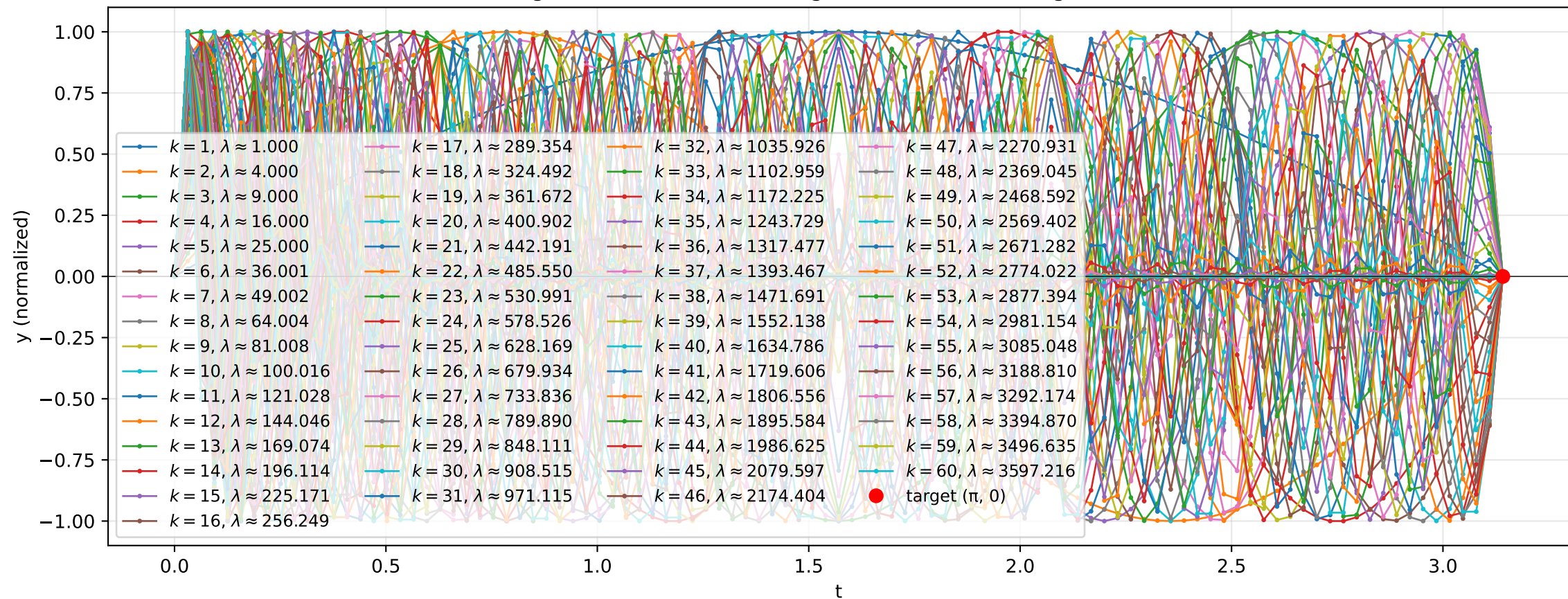
Eigenfunctions on uniform grid (n=100) for 60 eigenvalues
